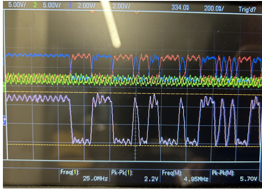
Fig. 6: Measured differential waveforms at 25 MHz test frequency. The yellow and green traces are the differential clock positive and negative lines, respectively. The blue and red traces are the differential data positive and negative lines, respectively. The purple trace shows the result of subtracting the differential data lines ( \text{DATA\_P} - \text{DATA\_N} ), clearly displaying the digital signal transitions. Signal quality at this frequency validated our design, though we operate at 20 MHz for our final implementation.
