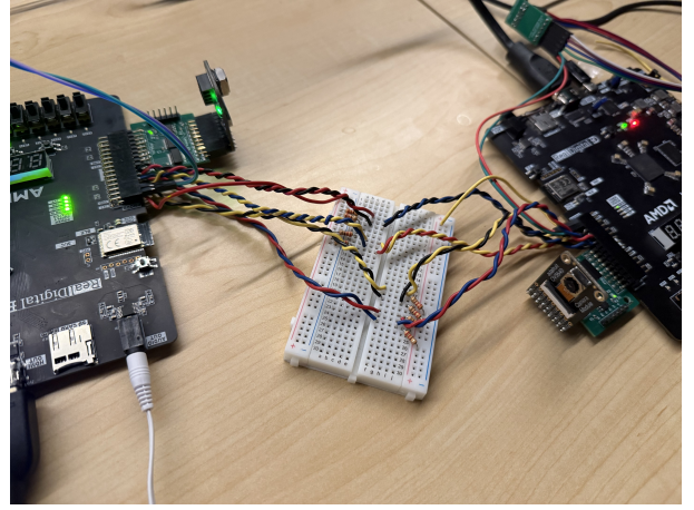
Fig. 2: Complete wiring setup showing both Urbana FPGAs connected via PMOD B cables with external pull-up resistor networks, cameras, HDMI outputs, and microphone connections.
