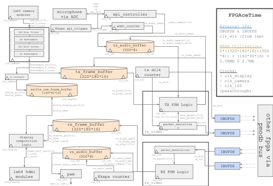
Fig. 7: System block diagram showing the complete bidirectional audio/video data flow. Both FPGAs operate identically, with simultaneous transmit and receive pipelines.
