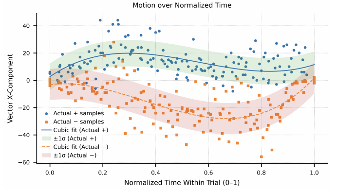
Fig. 6. Time-normalized trajectories of the measured x-component during repeated rest-to-rest harmonic motion trials.
