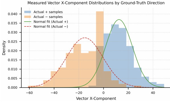
Fig. 5. Empirical distributions of the measured x-component conditioned on known positive and negative motion directions.
