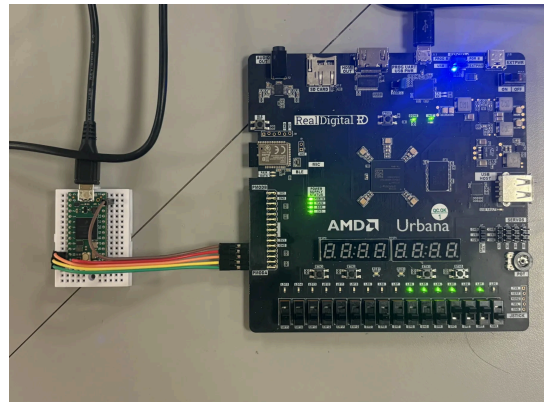
Fig. 4. SPI Hardware Setup.
