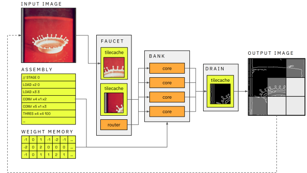
Fig. 1. High-level system flow.
