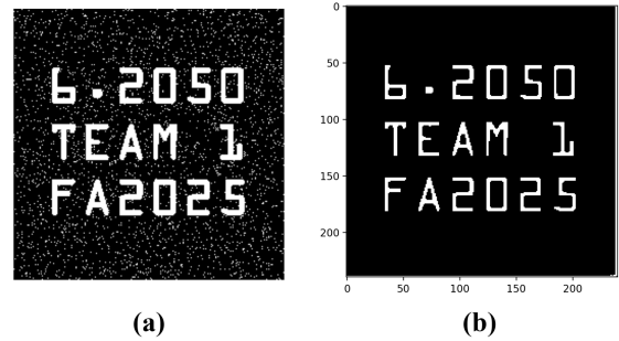
Fig. 7. (a) Noisy input cleaned by FPGA with one iteration of erosion, producing output image (b).
