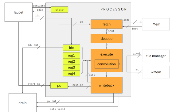
Fig. 3. Processor core diagram.
