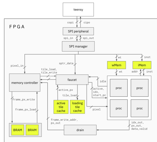
Fig. 2. High-level system architecture.
