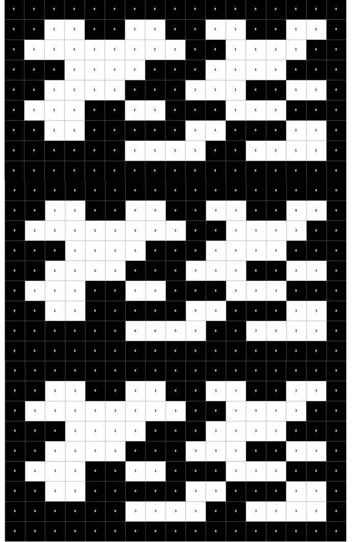
Fig. 1: Example walkthrough of connected components labeling algorithm [2].
