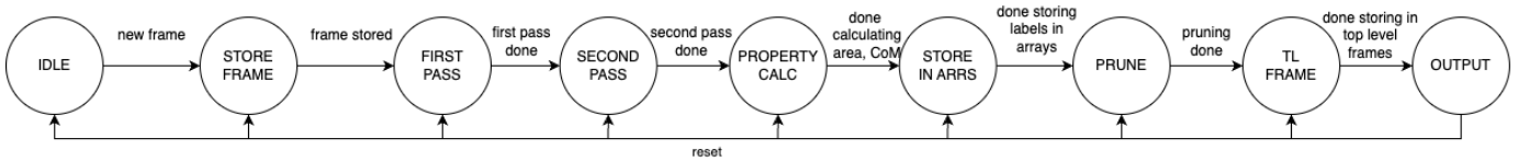
Fig. 6: FSM diagram for Connected Components Labeling module
