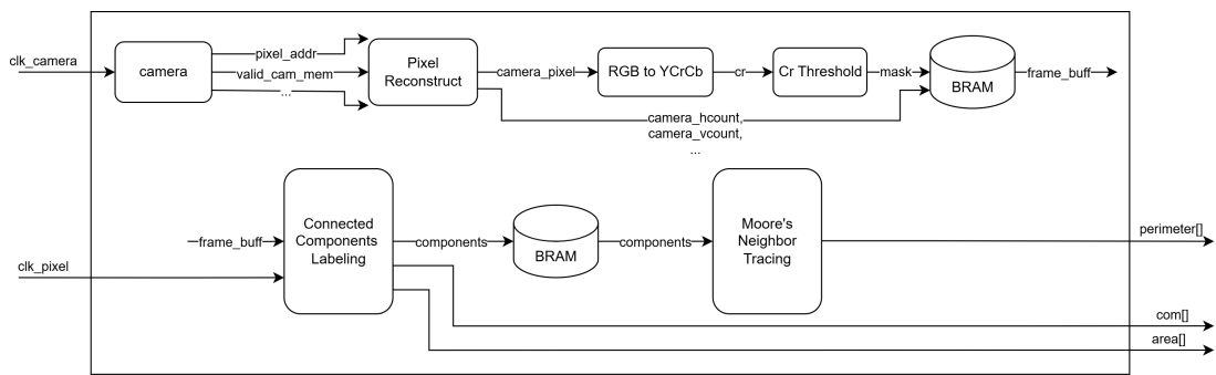
Fig. 5: Block diagram for image processing
