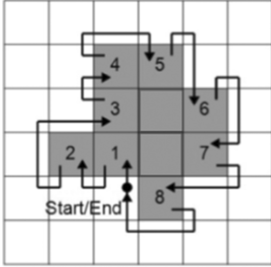
Fig. 2: Example walkthrough of Moore's Neighbor Tracing algorithm [4].
