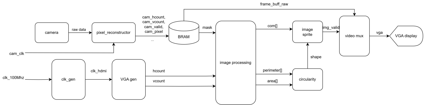
Fig. 4: Block diagram of top level module
