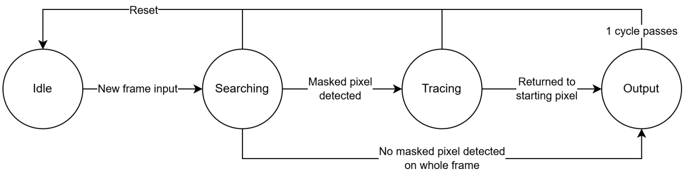
Fig. 7: FSM diagram for Moore's Neighbor Tracing module
